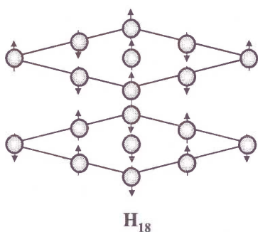
Enhanced Antiferromagnetic State by Artificial Elongation for Hydrogen Clusters
