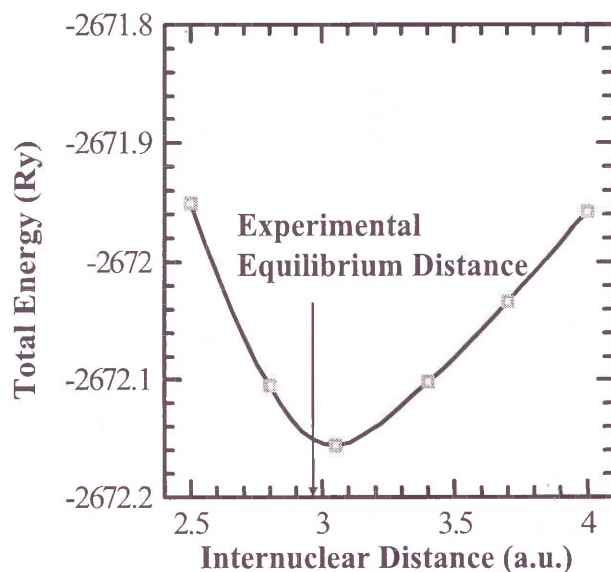
Calculated Total Energy for FeO
