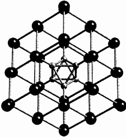
Boron cluster with octahedron composed of six borons in silicon.
